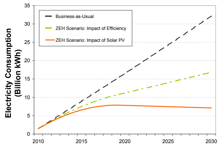
Figure 8: Texas New Home Electricity Consumption under the Net-Zero Energy Homes Scenario
