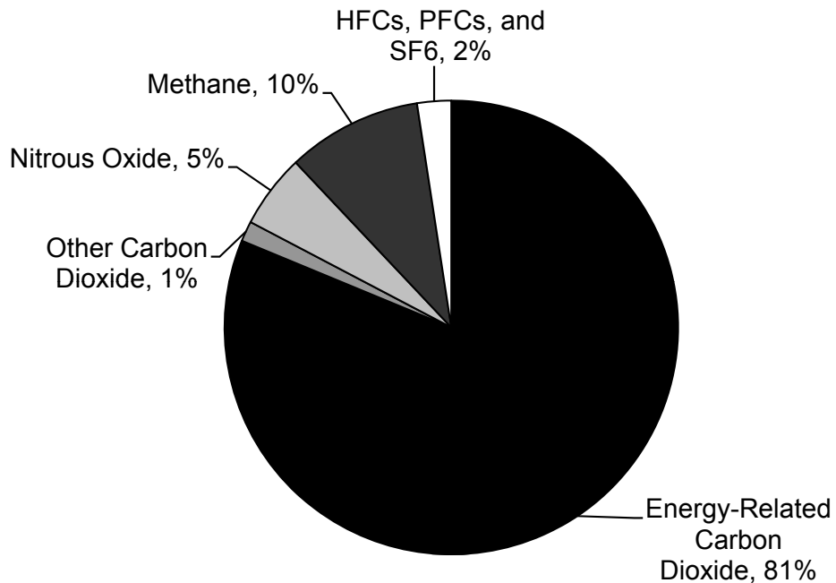
Figure 3. U.S. Global Warming Emissions by Pollutant, 2007 12
